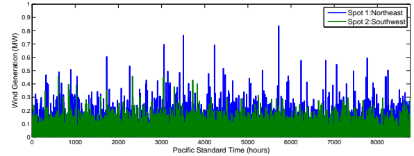
Figure 9. Wind power generation in Year 2013 on Jeju Island
