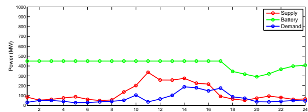
Figure 11. Supply, battery and demand curves on Jan 1st, 2013 on Jeju Island
